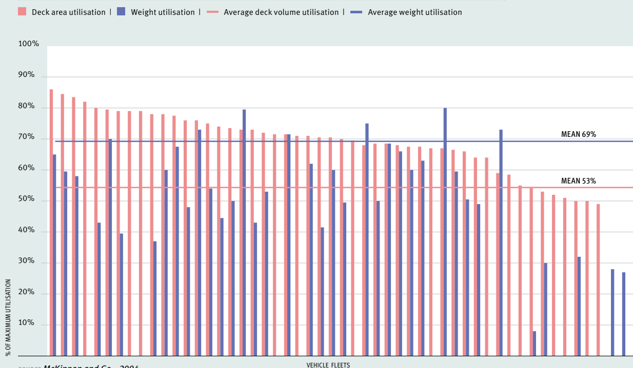
FIGURE 5: VARIATIONS IN WEIGHT AND DECK AREA UTILISATION ACROSS 53 TRUCK FLEETS
